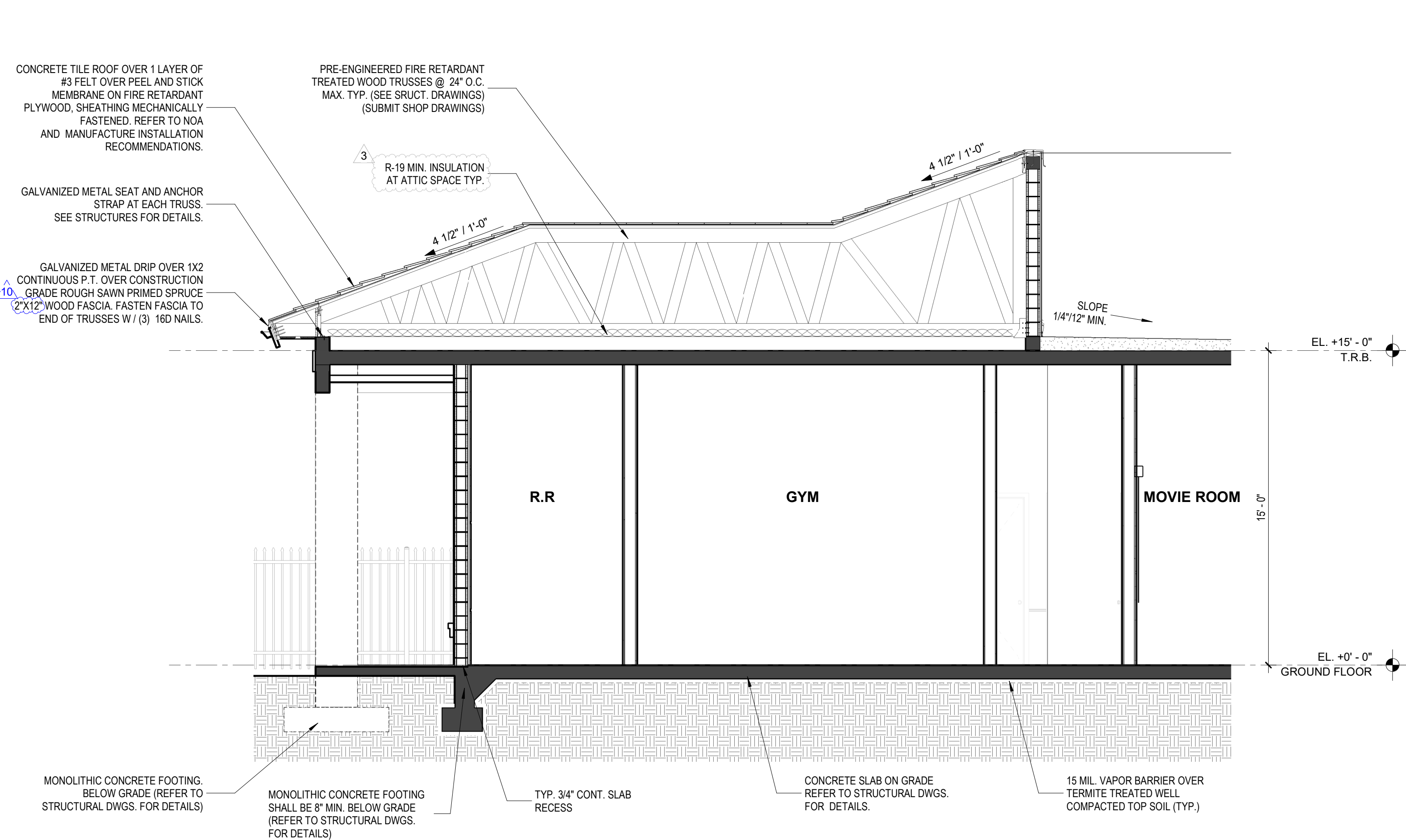
3 COMM. CENTER WALL SECTION 7 SCALE: 1/4" = 1'-0"
