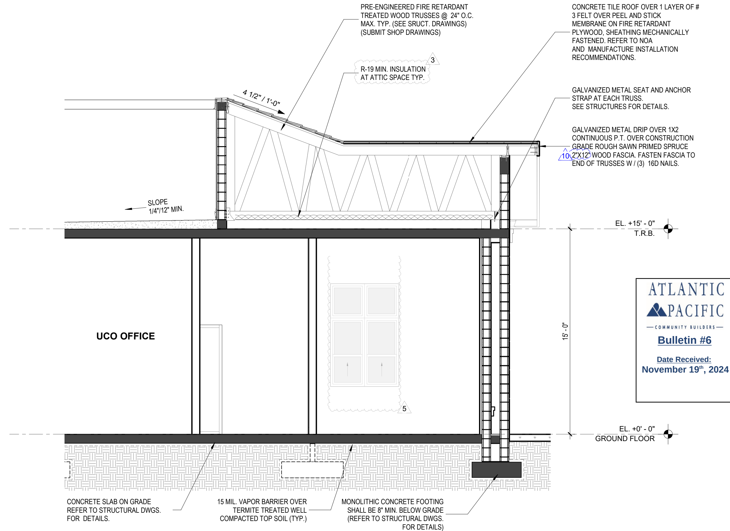
4 COMM. CENTER WALL SECTION 8 SCALE: 1/4" = 1'-0"
