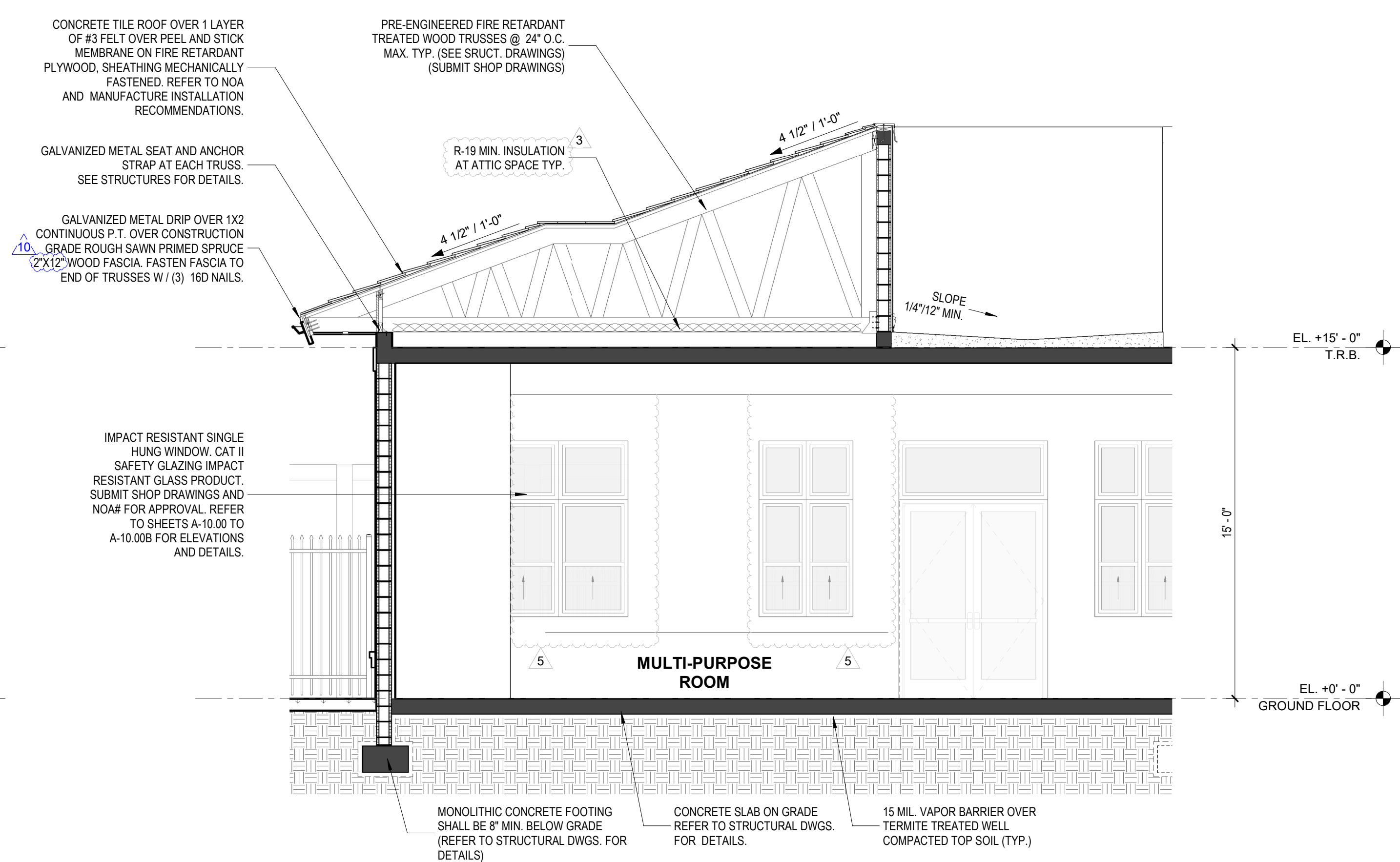
2 COMM. CENTER WALL SECTION 6 SCALE: 1/4" = 1'-0"
