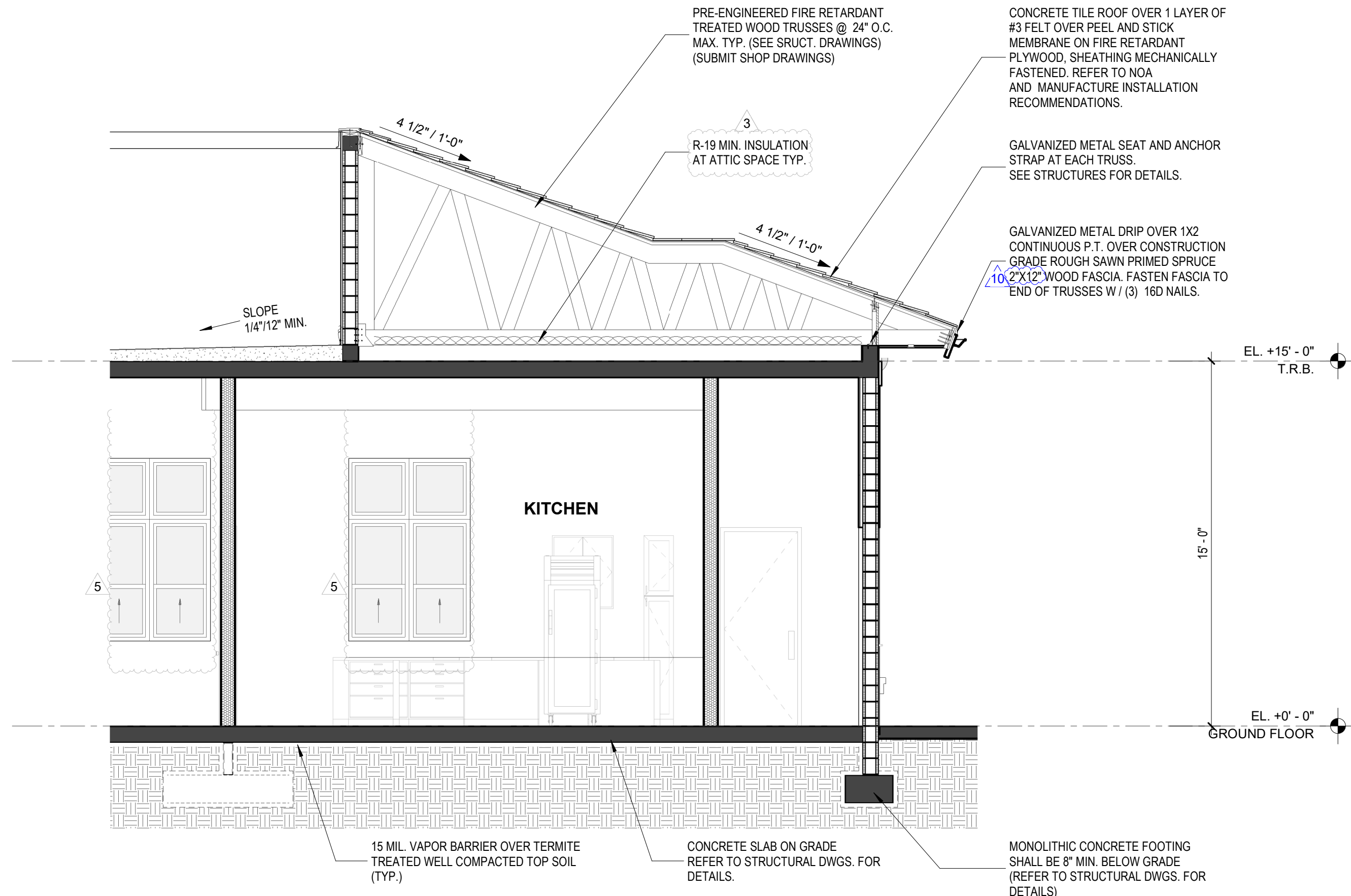
1 COMM. CENTER WALL SECTION 5 SCALE: 1/4" = 1'-0"
